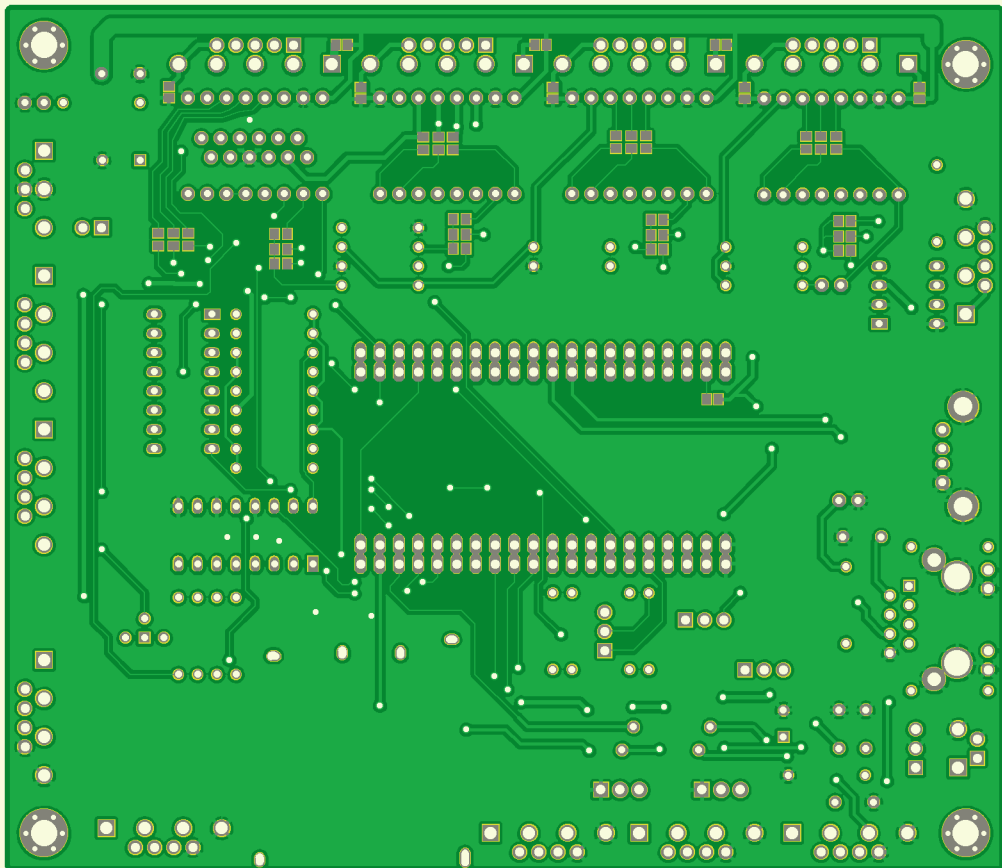
E453774 PCB view BOTTOM (bottomview)
