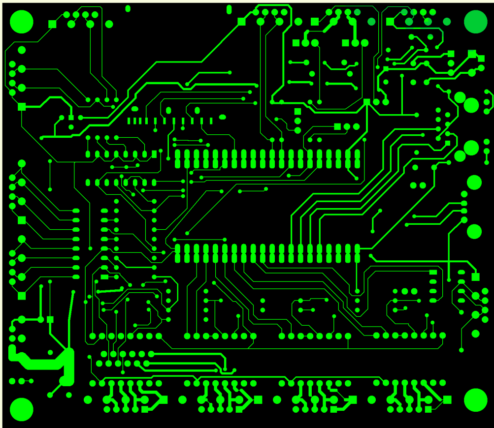
E453774 TOP layer Plating Image - PlatingIndex = 0.99 (topview)
